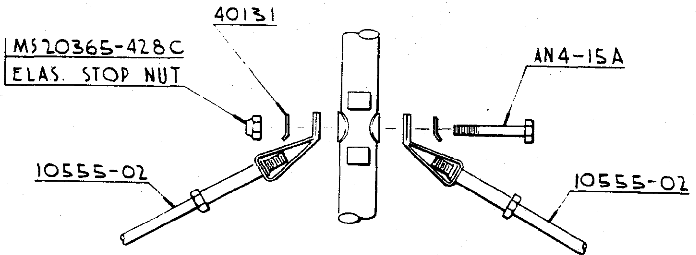
FIN TIE ROD ATTACHMENT
